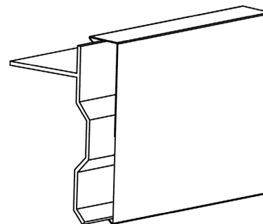
4-inch (102 mm) wide Gravel Stop with Metal Cover (see detail 3530)
