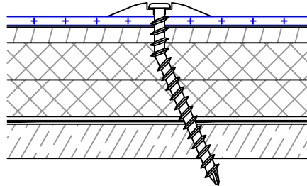
Fastener bent
