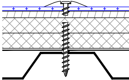
Fastener snapped
