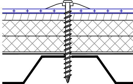
Fastener underdriven
