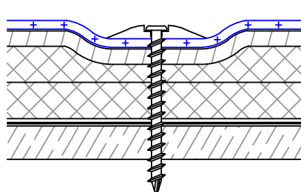
Fastener overdriven
